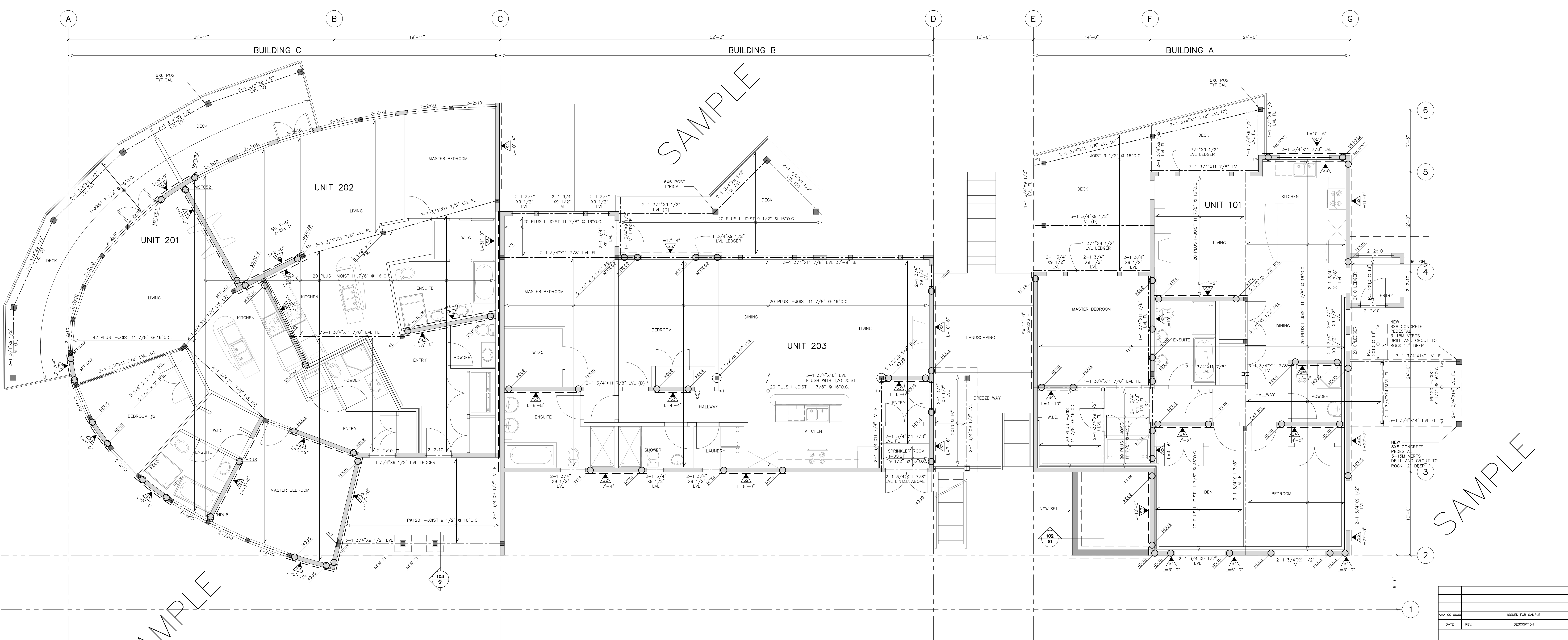
LEVEL 3 FLOOR FRAMING PLAN SCALE = 1/4" = 1'-0"
